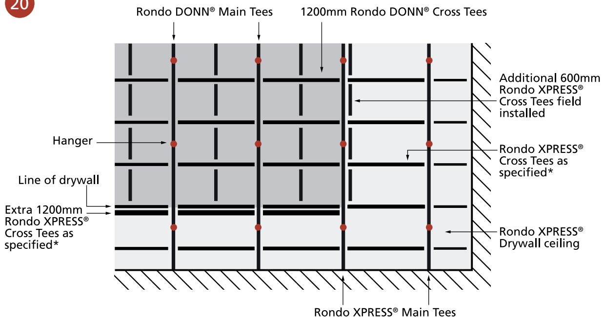
■ TYPICAL PLAN VIEW OF RONDO DONN® AND RONDO XPRESS® DRYWALL TRANSITION
