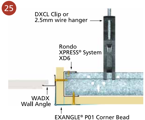
■ STANDARD OFFSET TRANSITION
