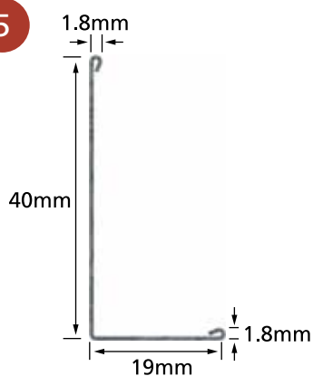
■ WAL LONG LEG WALL ANGLE – WAL
