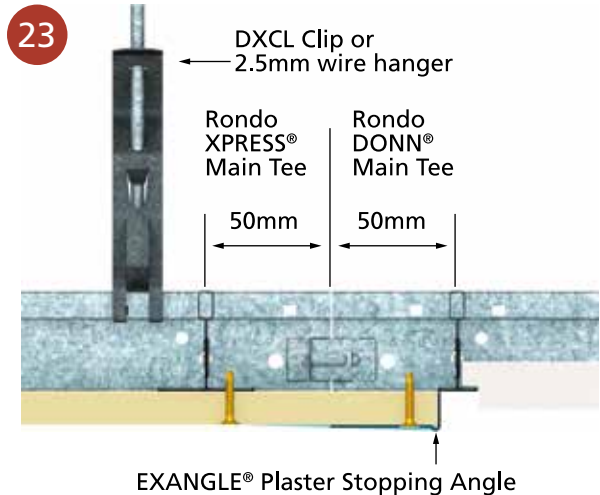
■ DRYWALL TO EXPOSED GRID TRANSITION: FACTORY END CONNECTION
