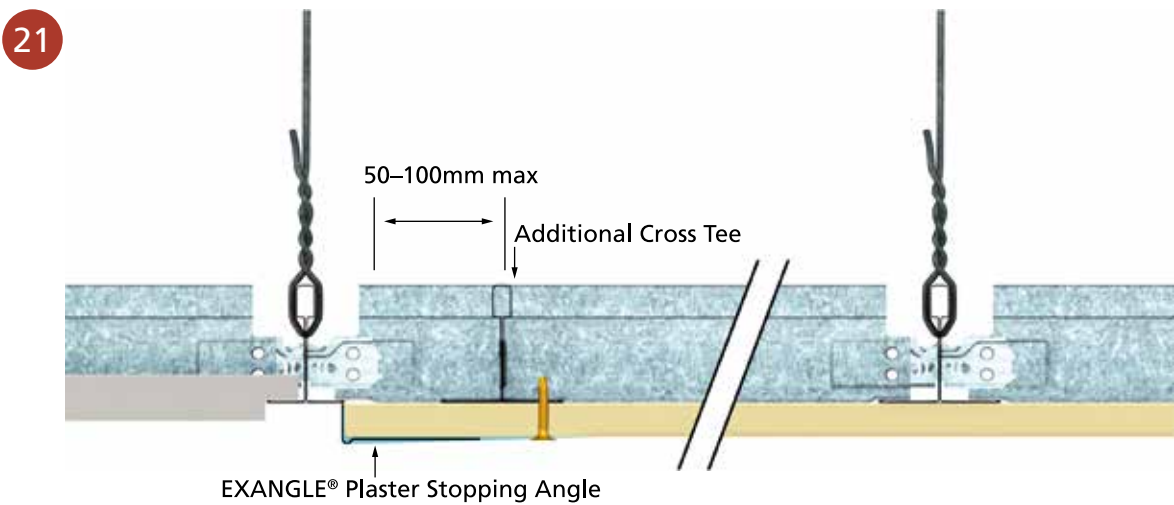
■ RONDO DONN® EXPOSED GRID TRANSITION TO RONDO XPRESS® DRYWALL GRID
