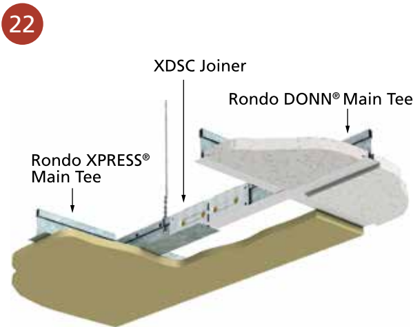
■ DRYWALL TO EXPOSED GRID TRANSITION: SITE CUT CONNECTION
